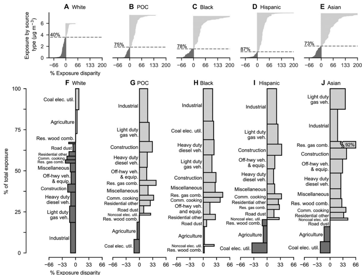
Figure 1. Source Contributions to Racial-Ethnic Disparity in PM 2.5 Exposure
