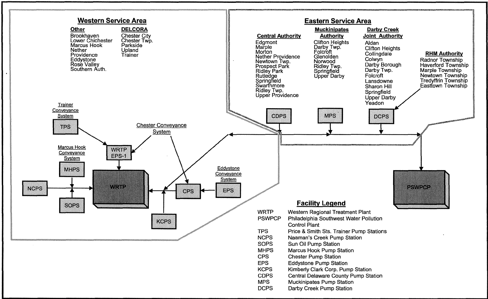
FIGURE 1-2 DELCORA's CONVEYANCE SYSTEM
