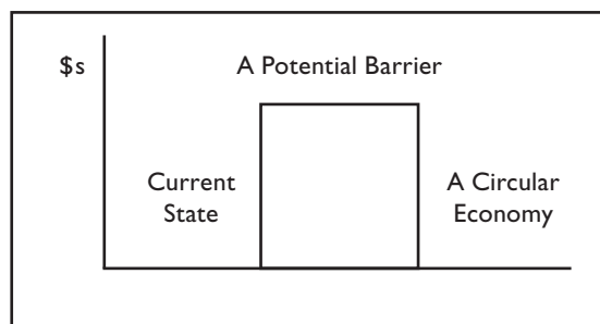
Figure 4: Potential Barrier
